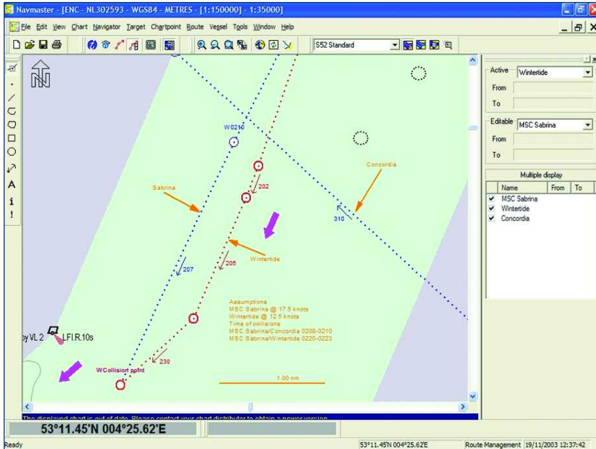
A reconstruction of the collision between Wintertide and MSC Sabrina (taken from the Marine Accident Investigation Branch report).
